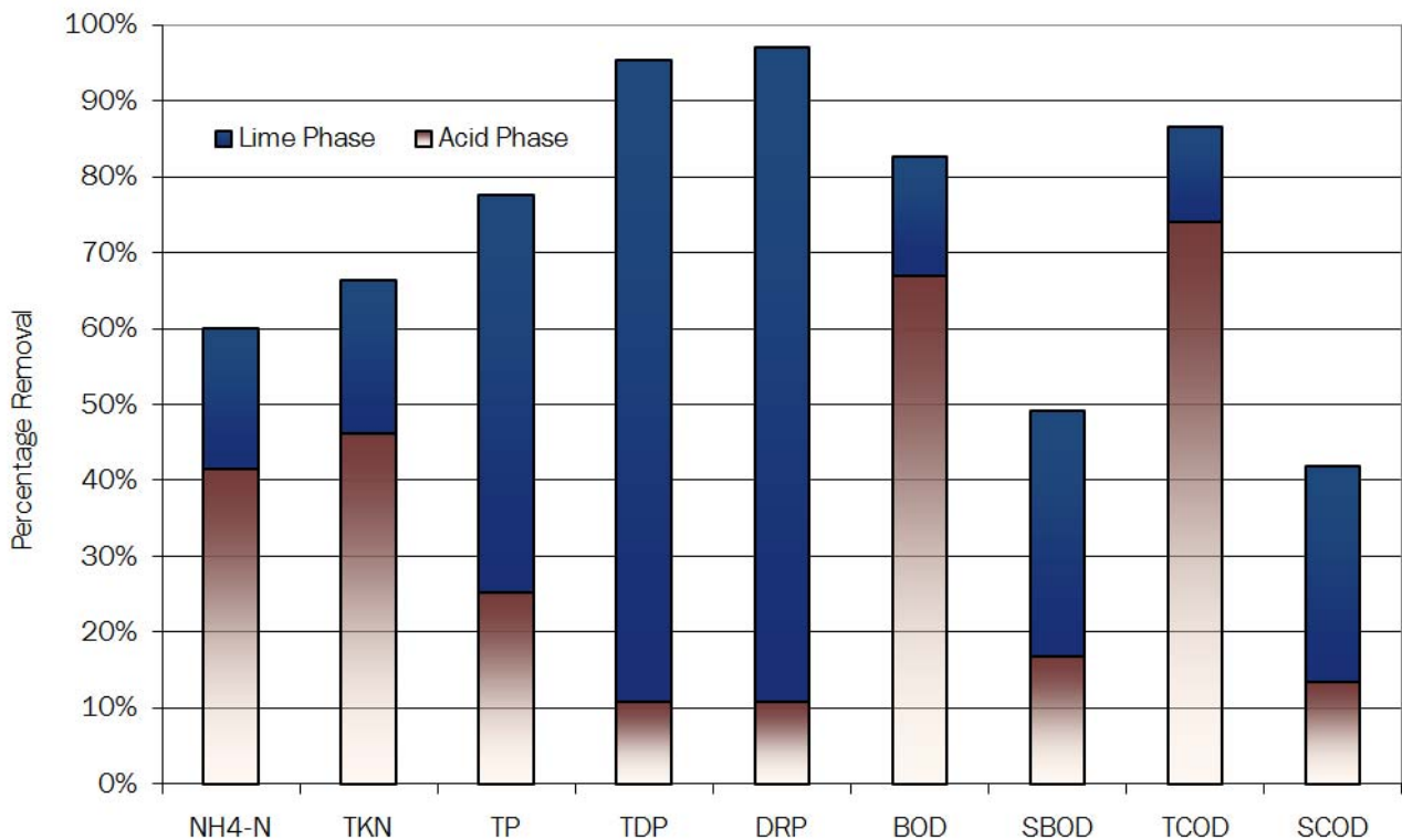
Figure 3: Typical Contaminant Removal in DAF-in-Series Patented System
